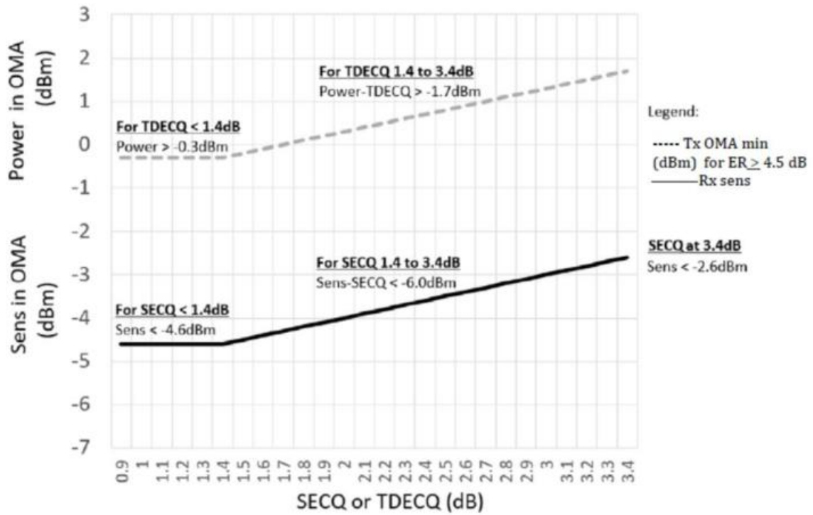
Illustration of Receiver Sensitivity Mask for 400G-FR4
