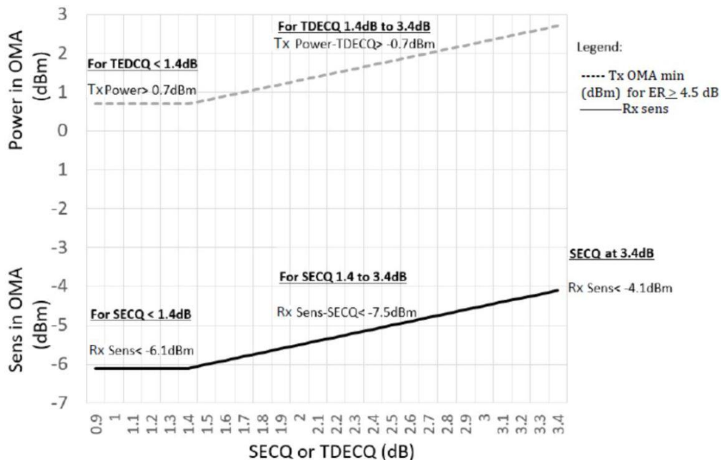
Figure 1. Illustration of receiver sensitivity mask for 100F-LR
